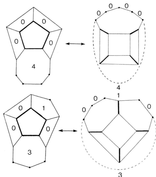
Fig. 3. Two pairs of corresponding systems. Left column : class Q_5 ; the numerals indicate numbers of vertices of degree two (symbolized by black dots) as distributed between consecutive vertices of degree three. Right column : class Q_4 ; the numerals indicate numbers of vertices of degree three as distributed between consecutive vertices of degree two (black dots).
