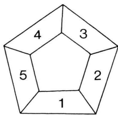
Fig. 1. The smallest system of the class Q_5 ( h=0 ).
